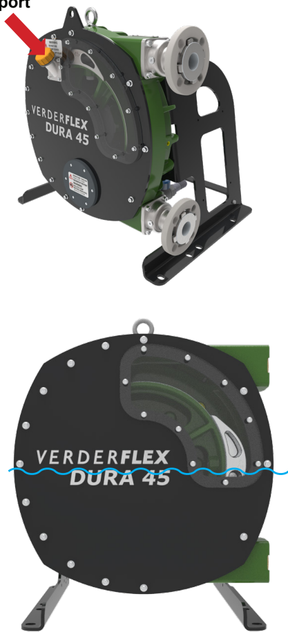
Figure 9. - Dura 45 lubricant - approximate fill level shown (7 litres)
