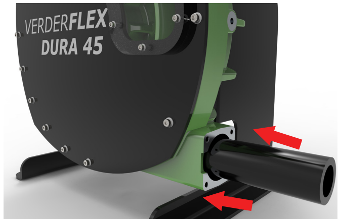
Figure 7. - Installing the hose
