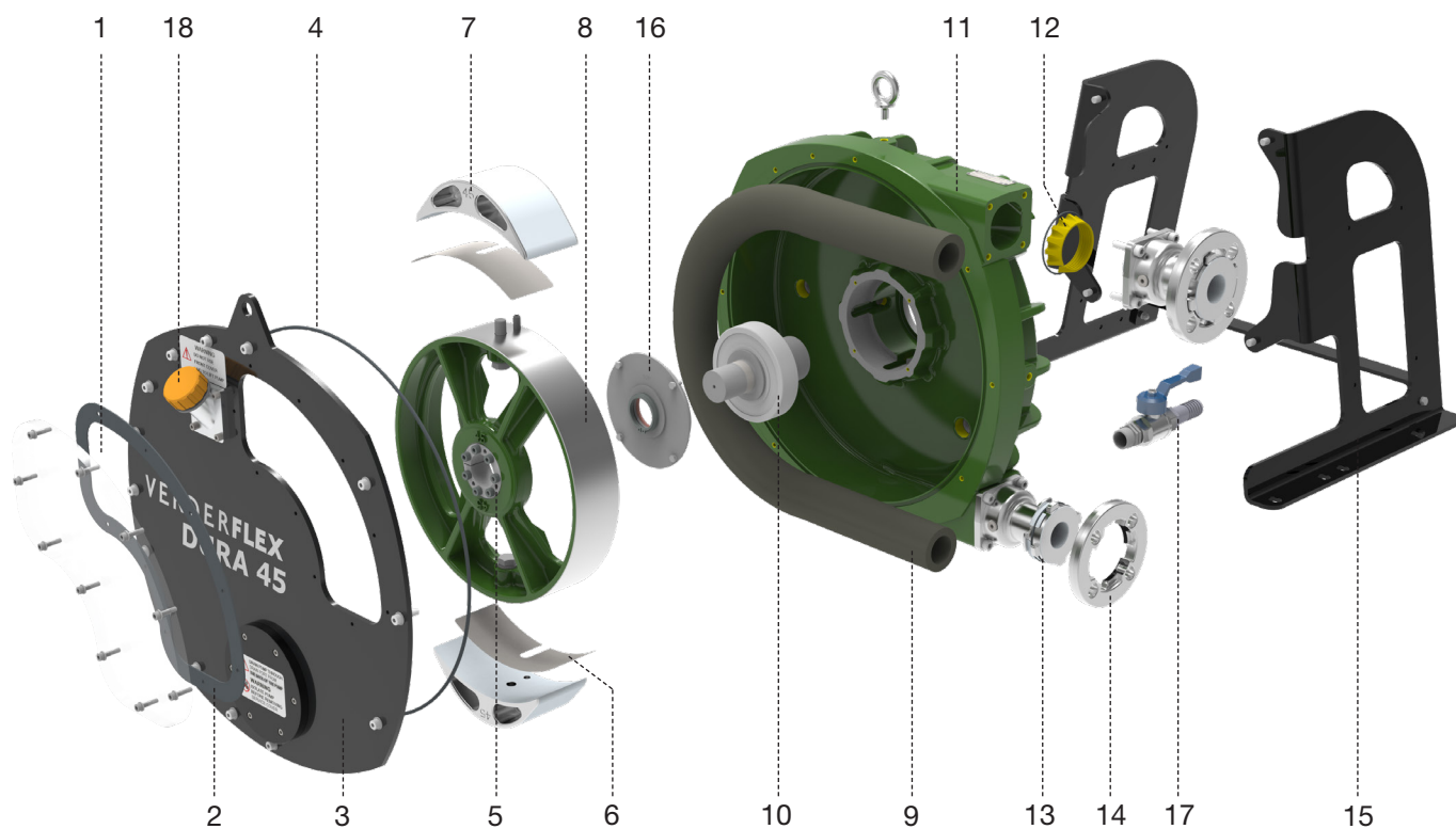
Figure 3. - Layout of Dura 45 Mk3 (generic view)
