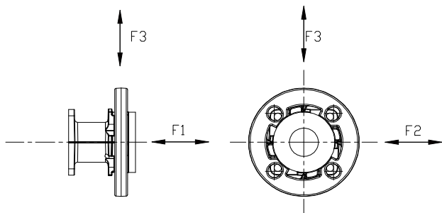
Figure 11. - Nozzle loadings on flanges
