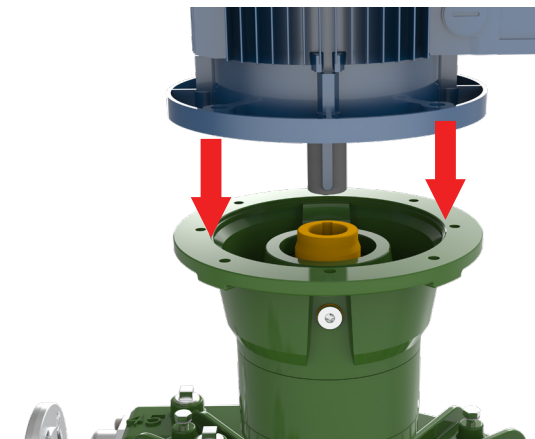
Figure 5. - Installing the motor
