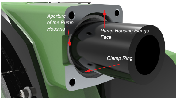
Figure 8. - Clamp ring inserted
